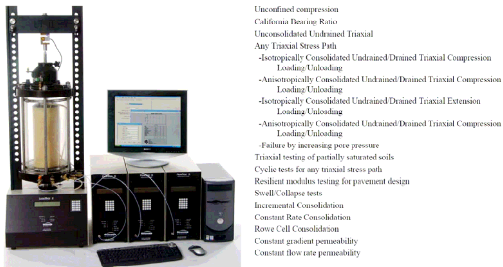
Figure 2: Geocomp Universal Test Station - Type I
