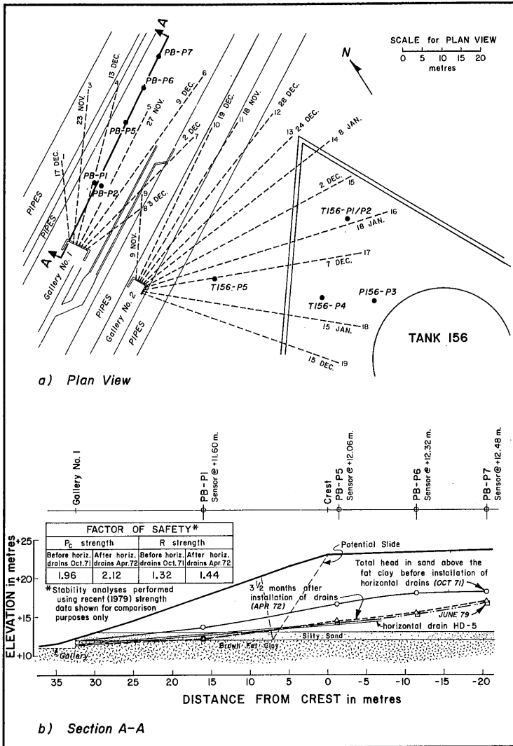
Fig. 14. Cliffside stabilization with lateral drainage.
