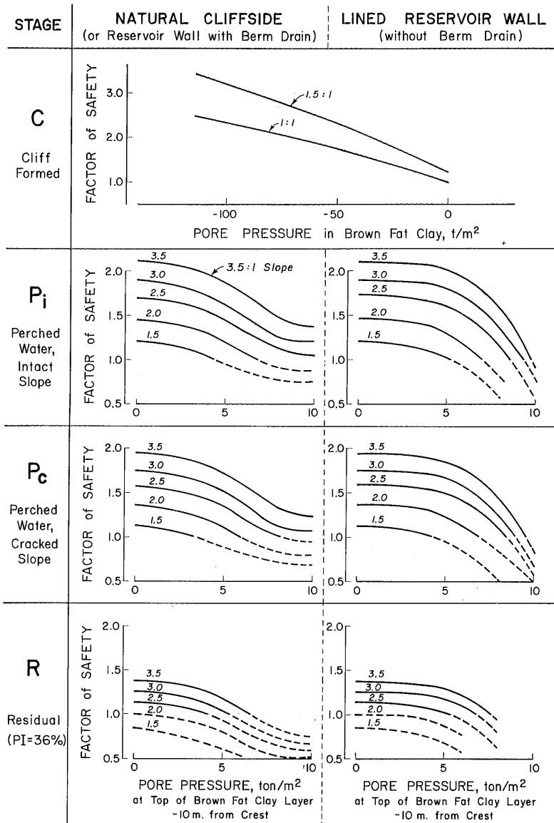
Fig. 11. Stability charts.
