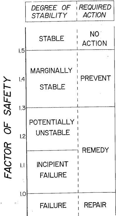
Fig. 12. Required action as function of degree of stability.
